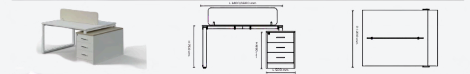
Extended Dimension: L 1400/1600 x D 1200 x H 750 mm Drawer Side Dimension: L 500 x D 1200 x H 650 mm
