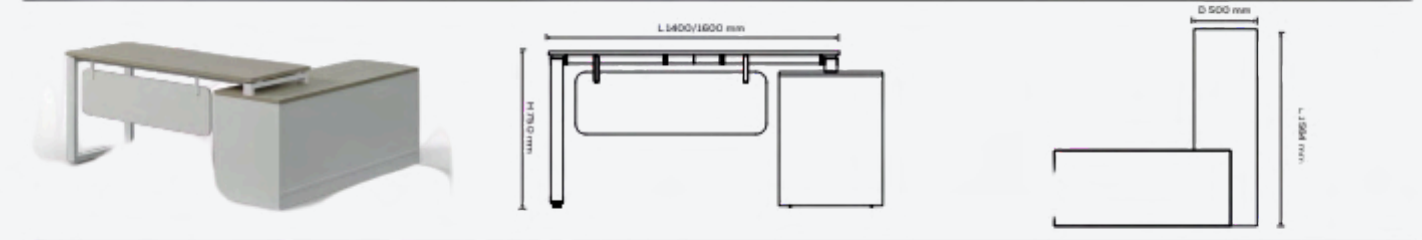
Desk Dimension: L 1400/1600 x D 600 x H 750mm Side Unit Dimension: L 554 x D 500 x H 650mm
