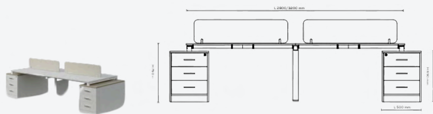
Extended Quadruple Workstation Dimension: L 2800/3200 x D 1200 x H 750 mm
