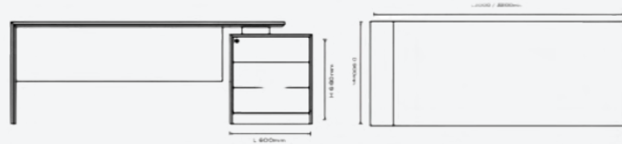
Drawer Side Dimension L 600 x D 900 x H 660mm
