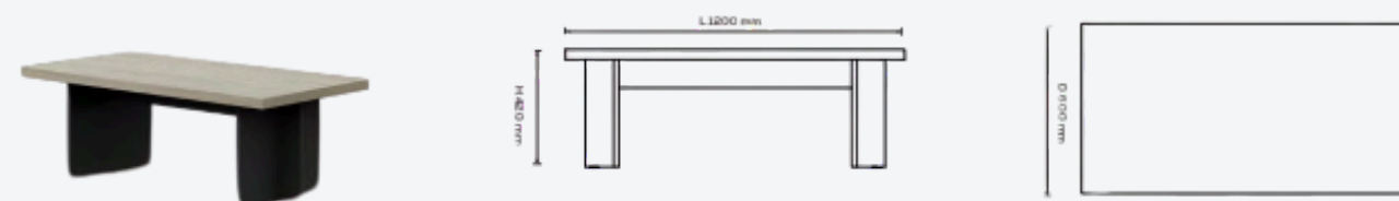
Coffee Table Dimension: L 1200 x D 600 x H 420 mm
