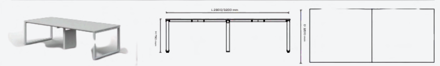
Extended Meeting Table Dimension: L 2800/3200 x D 1200 x H 750 mm
